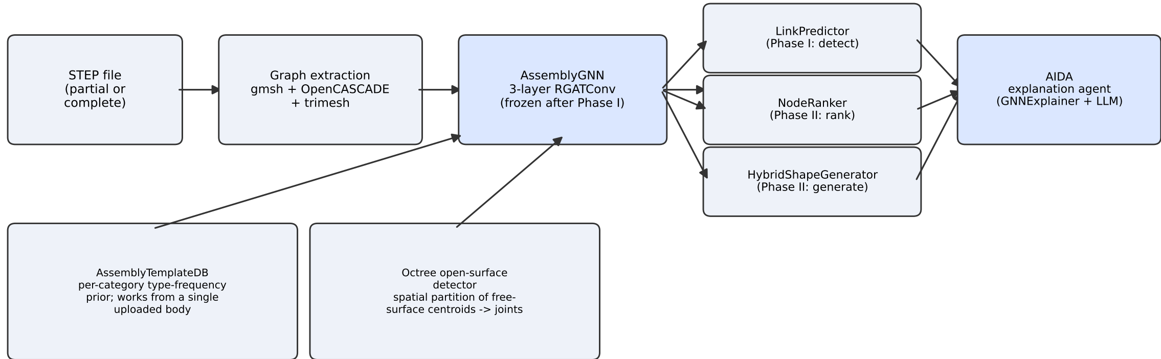
Fig. 1 System pipeline: one shared frozen encoder feeds three task heads and a live explanation layer.
